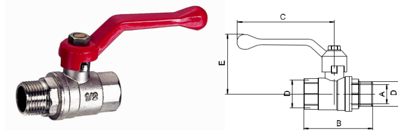
C.P. Ball Valve M.F With Lever Handle
