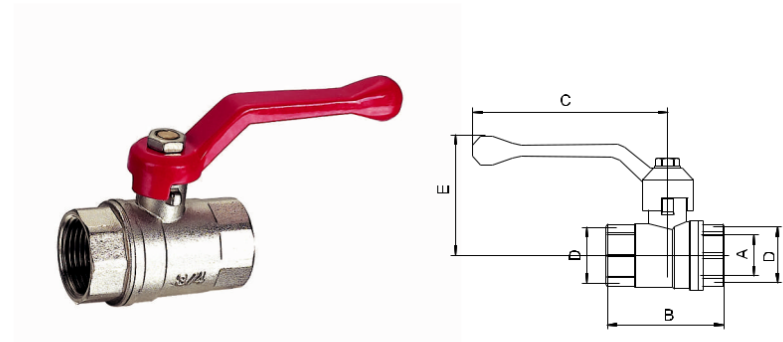
C.P. Ball Valve F.F With Lever Handle
